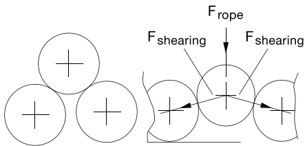
Figure 66 - danger of cutting in
