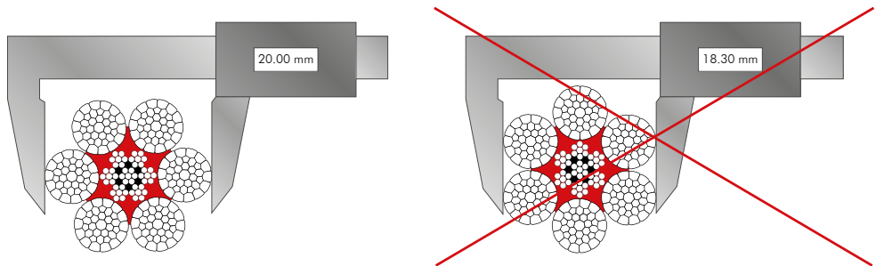
Figure 29 - Checking the diameter
