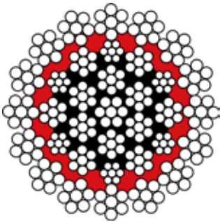
Figure 9 - Rotation resistant rope
