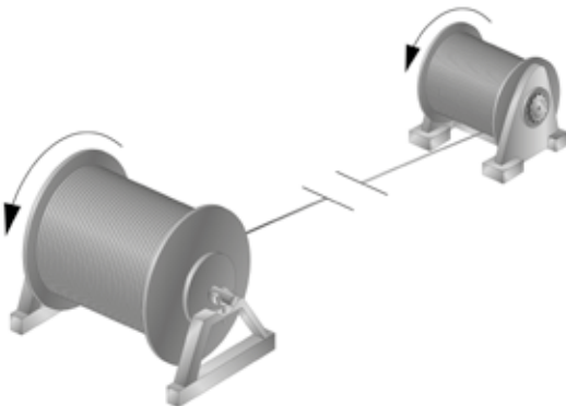
Figure 49 - correct method for locating the rope anchorage point on a drum
