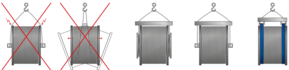
Figure 25 - Handling reels
