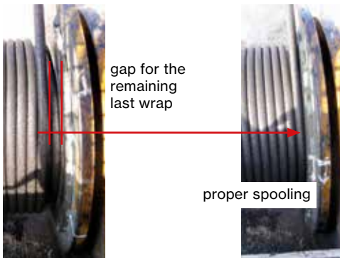
Figure 53 - proper spooling of first layer in order to avoid gaps to shim-plates that can cause rope crushing
