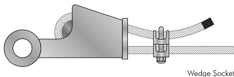
Figure 21b - Asymmetric wedge socket
