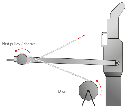
Figure 47 - side view: The fleet-angle between the reel and the first pulley/sheave is depending on the distance of those two components
