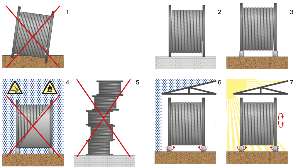
Figure 28 - Storage
