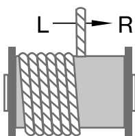
b) Left-hand-lay rope - underwind
