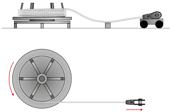
Figure 38 - Uncoiler
