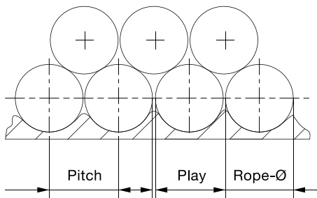
Figure 62 - \text{Play} = \text{Pitch} - \text{Rope-}\varnothing = (for a new applied rope)
