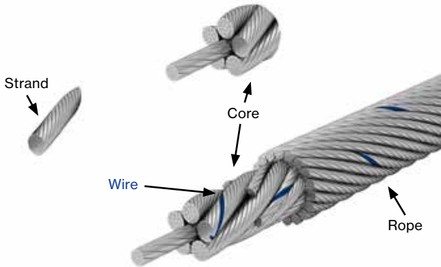
Figure 1 - Elements of a wire rope
