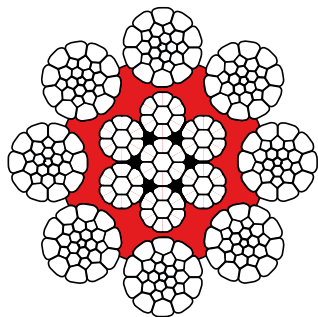
Figure 7 - EPIWRC
