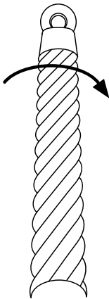
Figure 56 - example of a dead end: two different views, but one rope Figure 57 - Lay Type of rope: ordinary right
