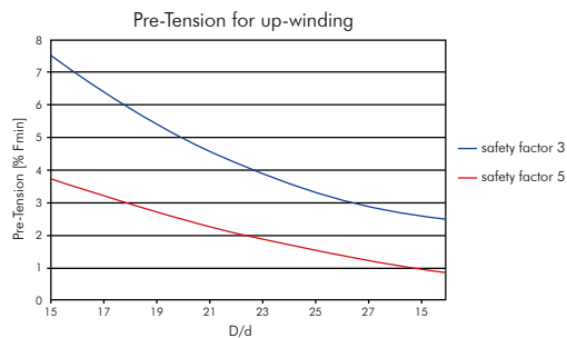
Figure 59 - relationship between pre-tensioning and D/d ratio of the drum
