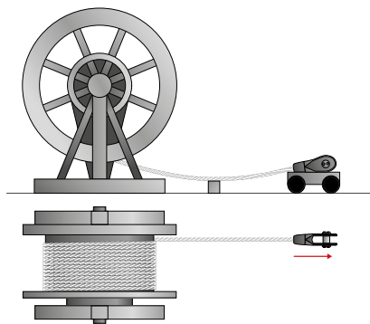
Figure 37 - Unreeeler
