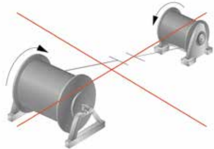
Figure 44 - incorrect tensioned unwinding using a winch
