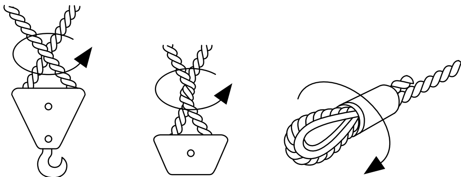
Figure 61 - how to untwist a hoisting rope
