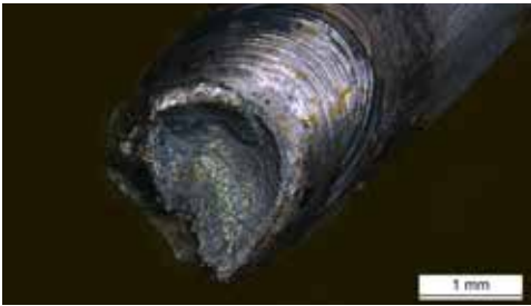
Figure 97 - Electric arcing
