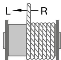
Figure 23 - correct method for locating the rope anchorage point on a drum
