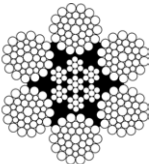
Figure 6 - Independent wire rope core (IWRC)
