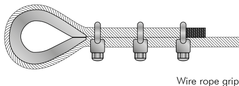
Figure 21c - U-bolt grips
