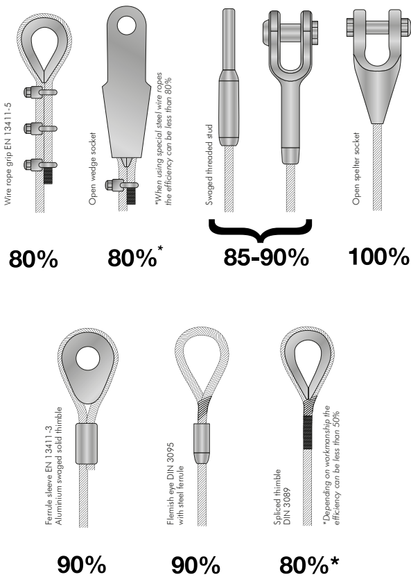
Figure 22 – Types of wire rope end terminations and respective efficiency factors
