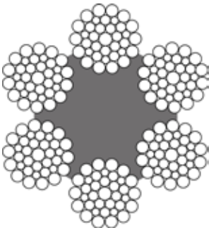
Figure 5 - Fiber cores (FC)
