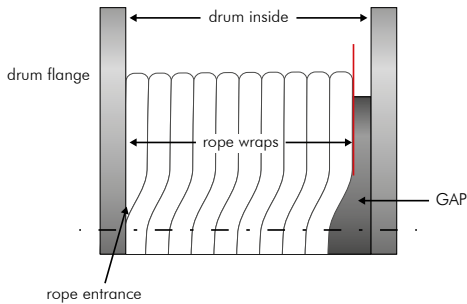
Figure 51 - gap check after first layer fully spooled on sheave
