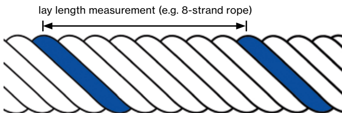
Figure 31 - Lay length measurement, direct method
