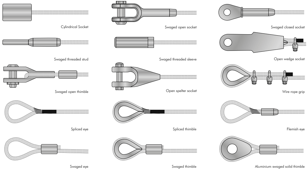
Figure 11 - Rope terminations
