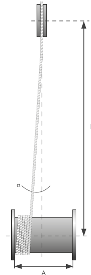
Figure 48 - top view of resulting fleet-angle depending on the distance of the reel and the first pulley / sheave
