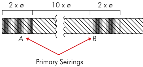
Figure 45 - Rope end with seizings
