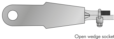
Figure 21a - Symmetric wedge sockets
