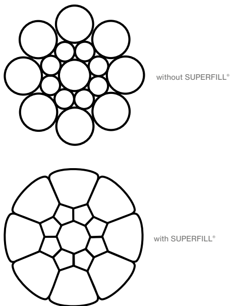
Figure 4 - SUPERFILL® compaction technology
