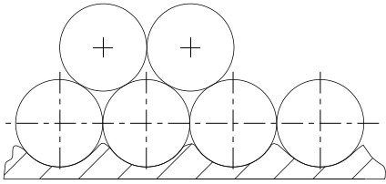
Figure 64 - No play between wraps results in addition wear
