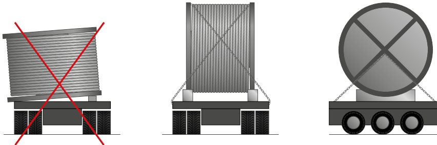
Figure 27 - Transport
