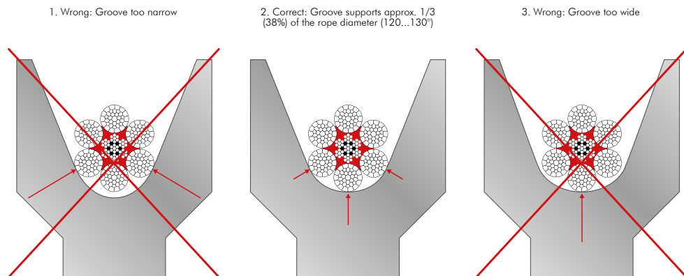
Figure 32 - Grooves
